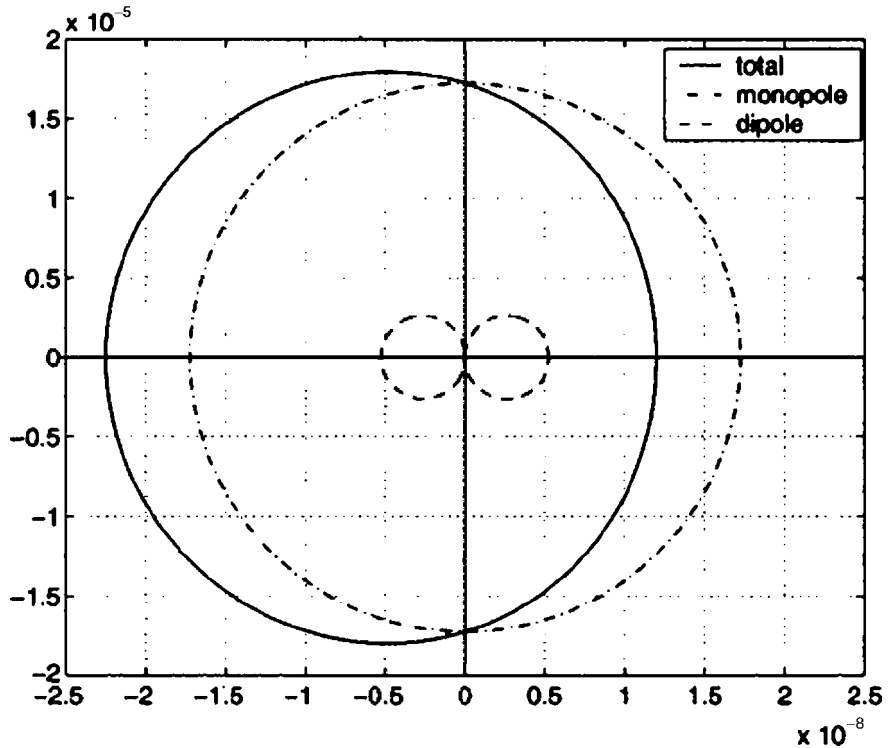
Figure 8.5 Contribution of the monopole (---) and dipole (----) terms of Eq. (8.2a) to the directivity pattern of the scattered field (—) produced by a red blood cell in water modeled as a fluid sphere for an incident plane wave coming in from the left (from Coussios, 2002, Acoustical Society of America).
