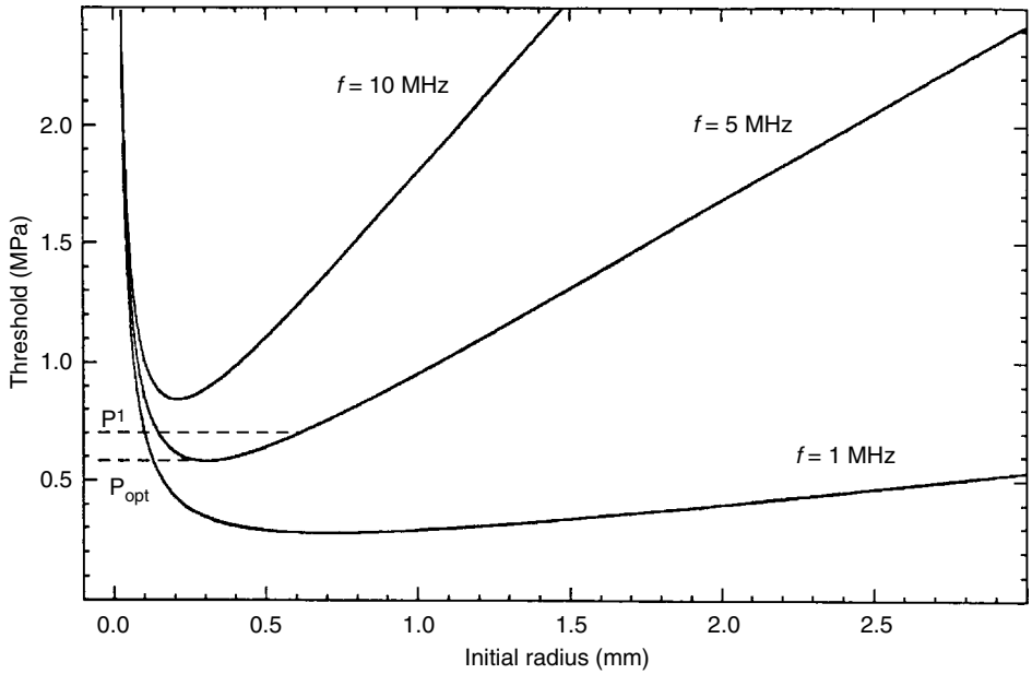
Figure 14.5 Peak rarefaction pressure threshold as a function of bubble radius for three frequencies ofinsonification: 1, 5, and 10 MHz. These curves represent inertial cavitation pressure amplitude thresholds (from Apfel and Holland, 1991, reprinted with permission from the World Federation of Ultrasound in Medicine and Biology).
