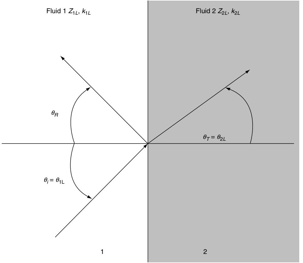
Figure 3.7 Oblique waves at a liquid–liquid interface.
