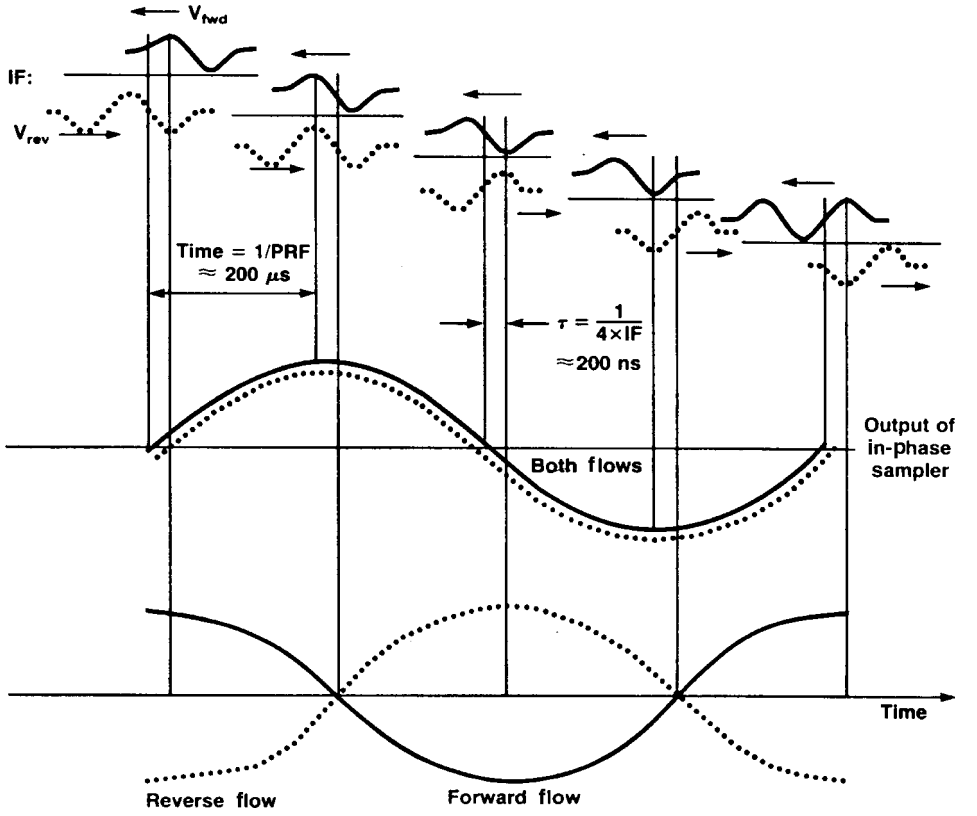
Figure 11.18 Quadrature sampling of forward and reverse flows for a pulsed Doppler system. (Top:) Echoes for five PRF intervals containing both forward and reverse flow Doppler time shifts. (Center:) Output of a single (in-phase) sampler for both echoes. (Bottom:) Output of second (quadrature) sampler allows differentiation of forward and reverse flows by phase encoding (from Halberg and Thiele, 1986, reprinted by permission of Hewlett Packard).
