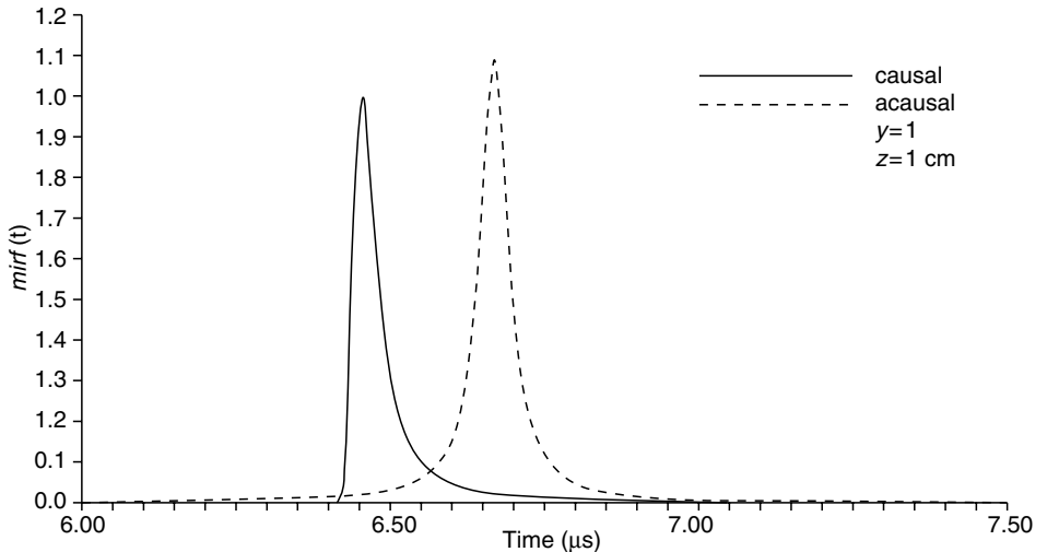
Figure 4.9 Comparison of causal time mirf and an acausal nondispersive mirf for linear loss ( y=1 ), for a propagation distance of 1 cm and an absorption coefficient of 0.1151 neper/MHz-cm (1 dB/MHz-cm) (from Szabo, 1993).
