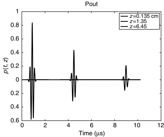
Figure 4.3 Changes in pressure-pulse shape of an initially Gaussian pulse propagating in a medium with a 1 \text{ dB}/\text{MHz}^{1.5}\text{-cm} absorption \gamma = 1.5 for three different increasing propagation distances ( z ).
