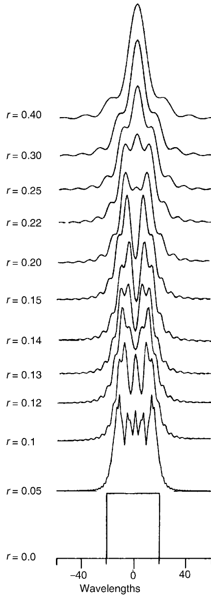
Figure 6.7 Diffraction beam profiles for different values of S = r with \hat{L} = 40(\lambda) . Profiles for other values of L can be found by scaling the profile at the appropriate value of S (from Szabo and Slobodnik, 1973).
