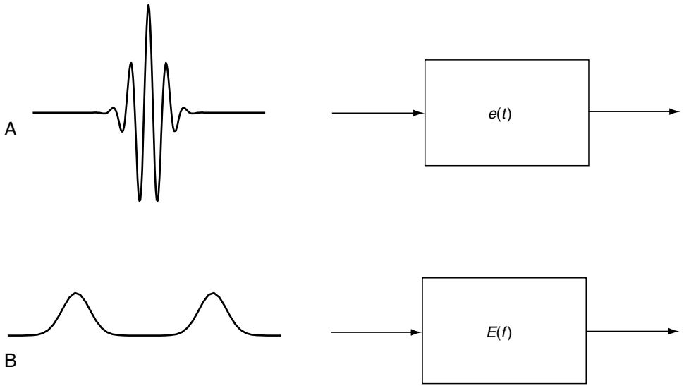
Figure 2.6 (A) A time domain building block and (B) its frequency domain equivalent.
