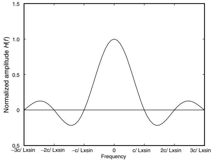
Figure 7.7 Far-field element directivity as a function of frequency for an element length L_x .
