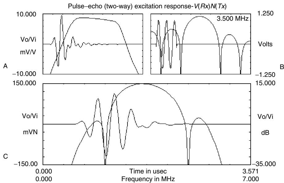
Figure 5.19 (A) Pulse-echo impulse response and spectrum for a 3.5-MHz linear array design. (B) A 3.5-MHz, 2½ cycle sinusoid excitation pulse and spectrum. (C) Resultant output pulse and spectrum. All calculations by PiezoCAD transducer design program (courtesy of G. Keilman, Sonic Concepts, Inc).
