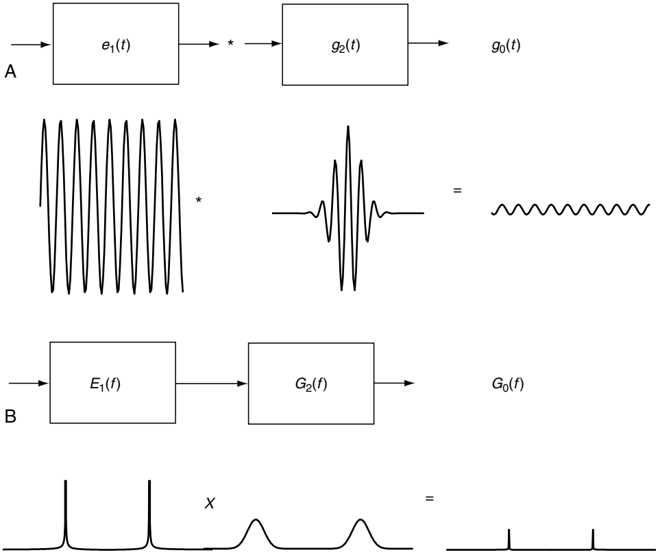
Figure 2.9 (A) Time domain filter output, to a 4.5-MHz tone input. (B) Spectrum magnitude of filter output is also at the input frequency but changed in amplitude and phase. The filter is centered at 5 MHz.
