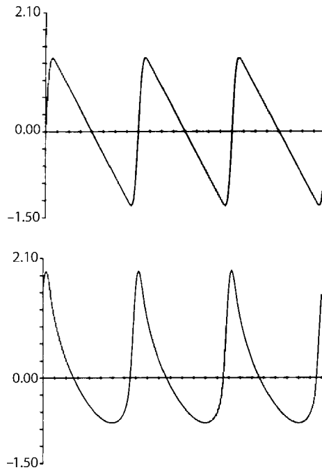
Figure 12.12 (Bottom) Waveform resulting from adding a constant phase of \phi = \pi/4 between harmonics in the standard Fourier series for a sawtooth (Top) (from Parker and Friets, 1987, IEEE ).
