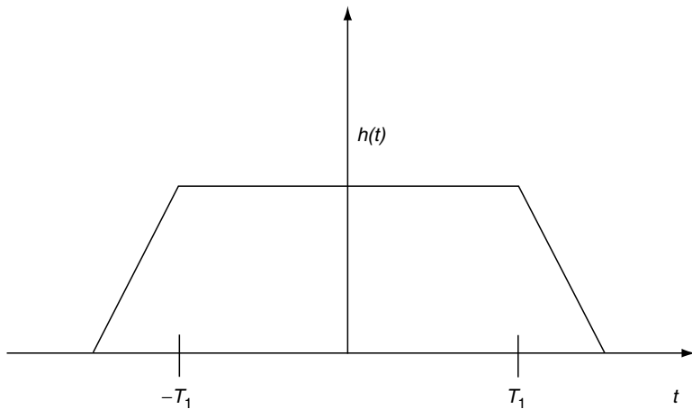
Figure 7.6 Trapezoidal far-field spatial impulse response for a rectangular array element.
