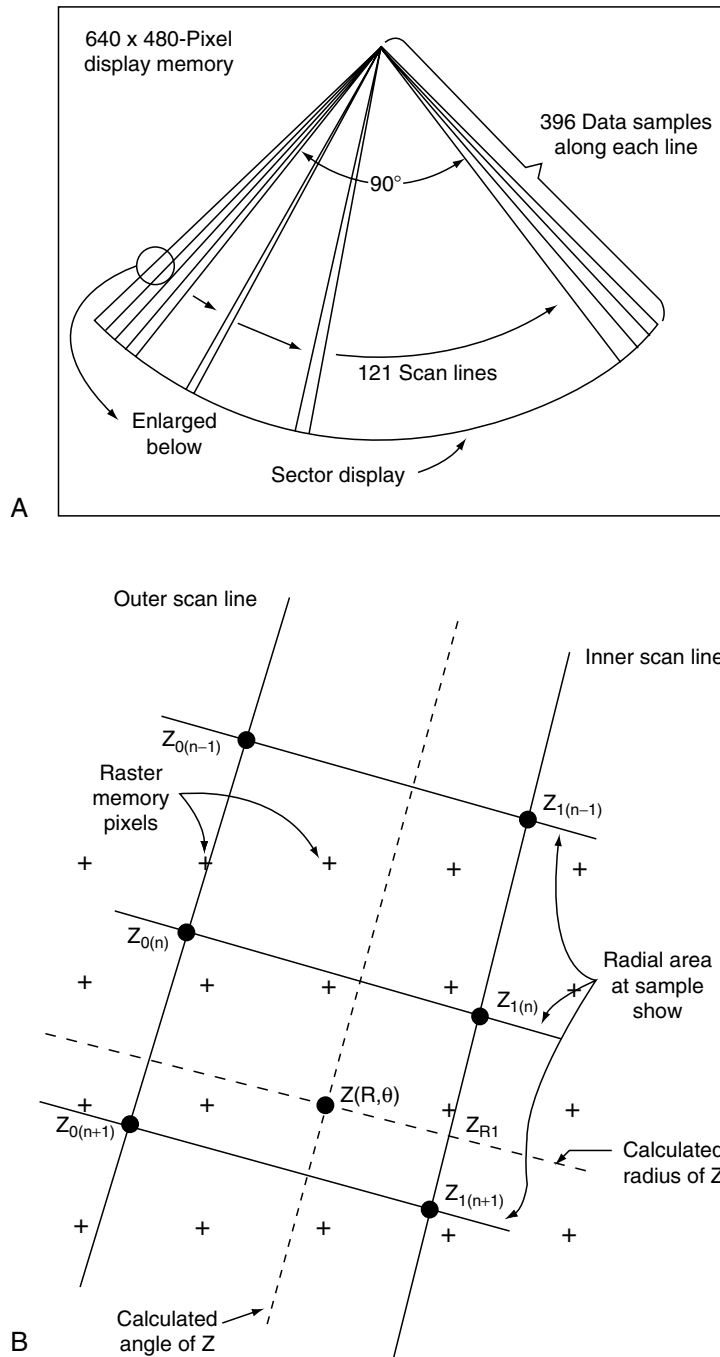
Figure 10.18 (A) Image vectors in a sector scan display overlaid on desired rectangle in format. (B) Magnified view comparing vector data in polar coordinates to rectangular pixel positions (Reprinted by permission of Hewlett Packard, from Leavitt et al. , 1983, Hewlett Packard).
