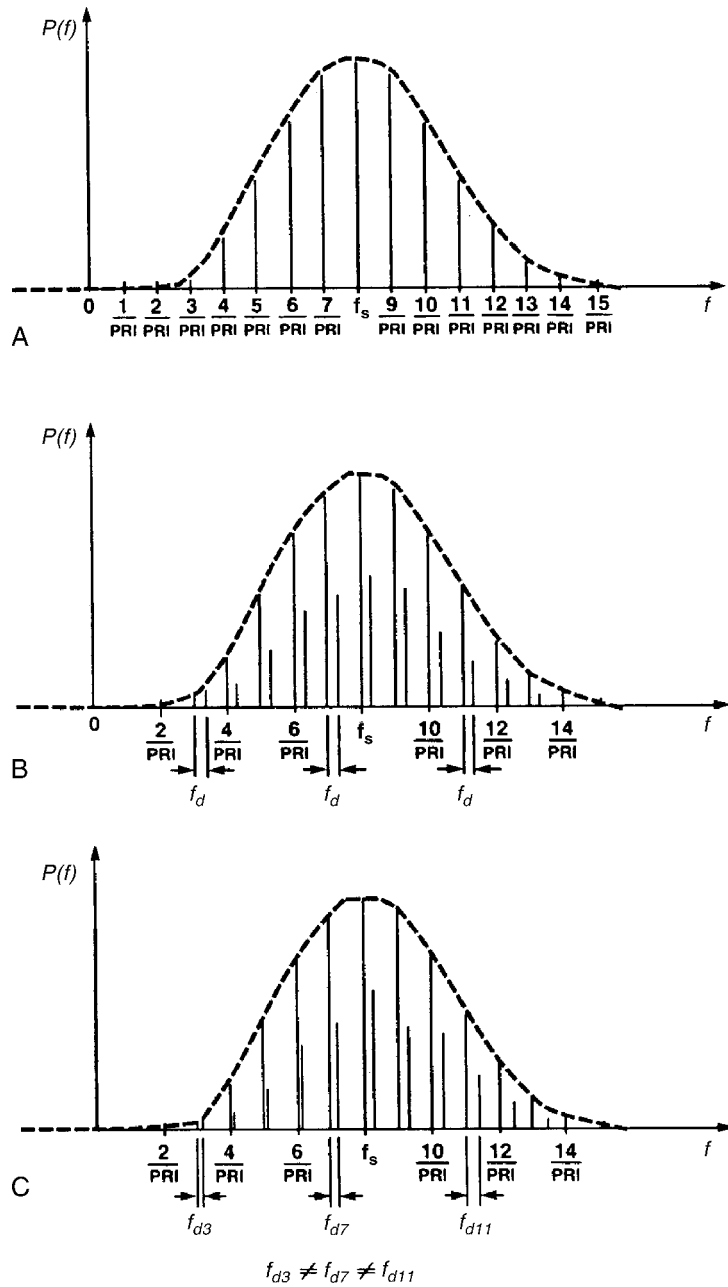
Figure 11.17 (A) Spectra of stationary objects for a Gaussian transmit pulse. (B) Equally shifted Doppler spectra compared to spectra from echoes from stationary objects. (C) Correctly shifted Doppler spectra compared to spectra from echoes from stationary objects (from Magnin, 1986, reprinted by permission of Hewlett Packard).
