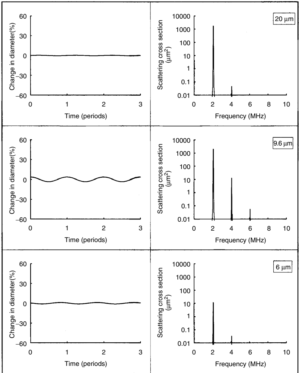
Figure 14.10 (Left panels) Simulated relative change in diameter of an Albnex bubble in water for a sinusoidal excitation of 2 MHz and a pressure amplitude of 50 kPa for three bubble diameters: 20 \mu\text{m} (above resonance), 9.6 \mu\text{m} (resonance), and 6 \mu\text{m} (half resonance). (Right panels) Corresponding spectral responses (from de Jong, 1993).
