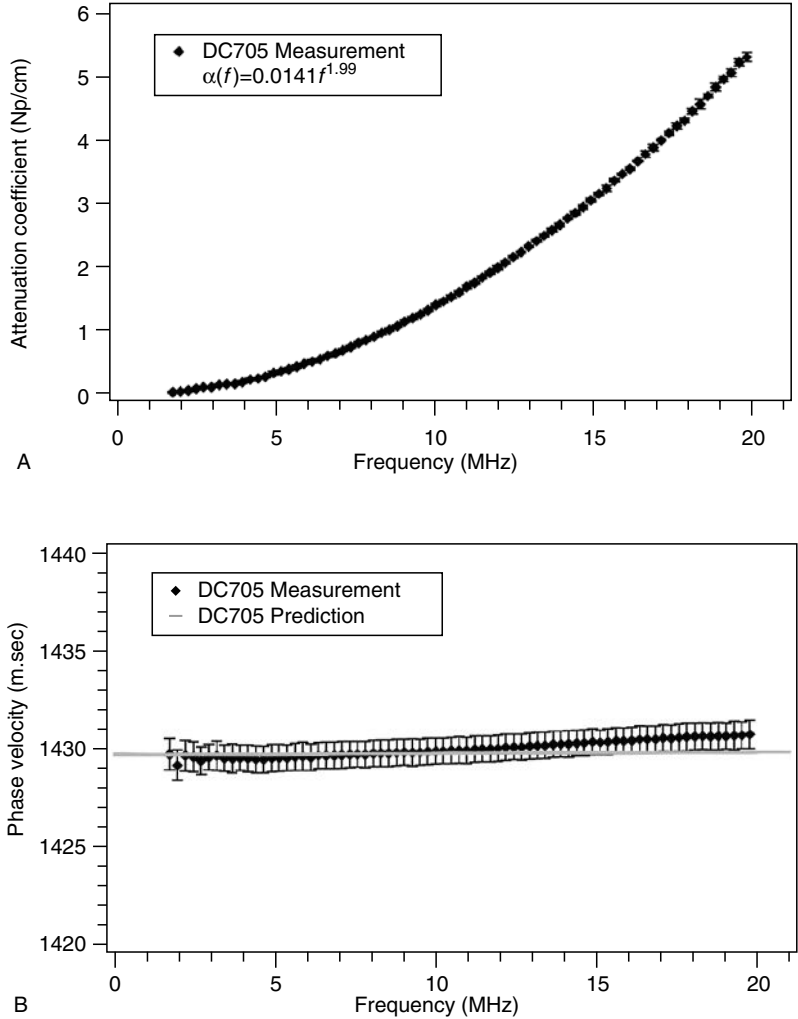
Figure 4.7 (A) Measured absorption data as a function of frequency for DC 705 (silicone fluid) with power law fit of \gamma \approx 2 . (B) Measured relative velocity dispersion with error bars compared to prediction from Eq. (4.19a) using the measured absorption data power law fit. Note that dispersion is nearly zero for this quadratic loss case (from Waters et al. , 2000a, Acoustical Society of America).
