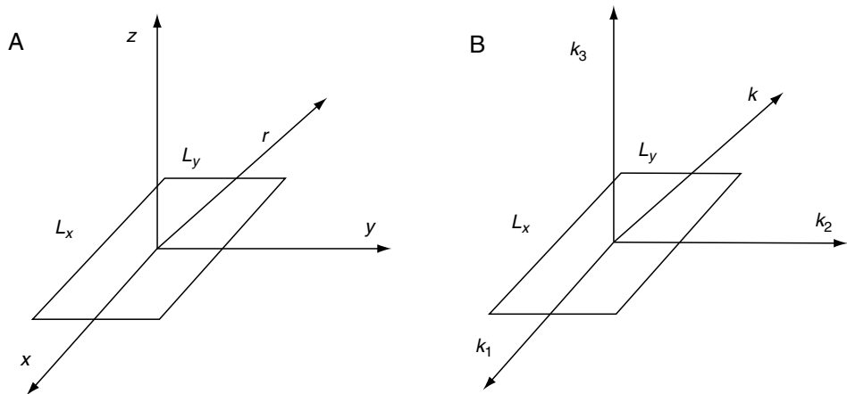
Figure 2.10 (A) Normal space with rectangular coordinates and a position vector r to a field point and (B) corresponding k -space coordinates and vector k .
