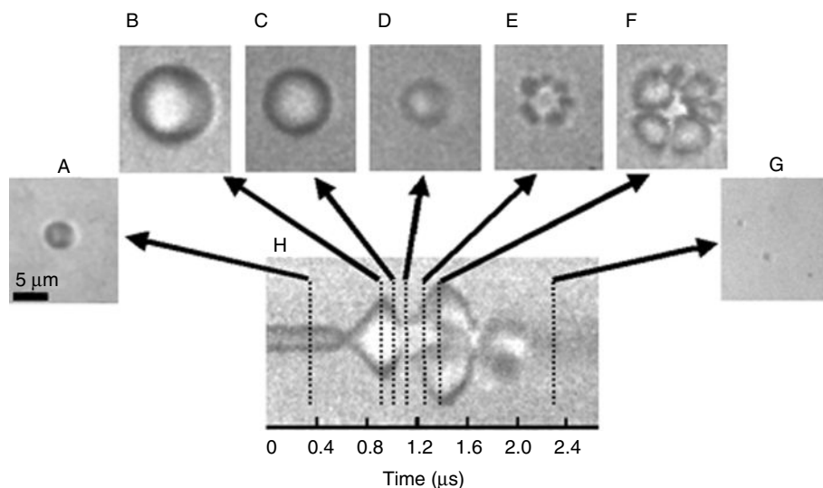
Figure 14.12 Optical frame images and streak image corresponding to the oscillation and fragmentation of a contrast agent microbubble, where fragmentation occurs during compression. The bubble has an initial diameter of 3\ \mu\text{m} , shown in (A). The streak image in (H) shows the diameter of the bubble as a function of time, and dashed lines indicate the times at which the two-dimensional cross-sectional frame images in (A)–(G) were acquired relative to the streak image (from Chomas et al. , 2000, American Institute of Physics).
