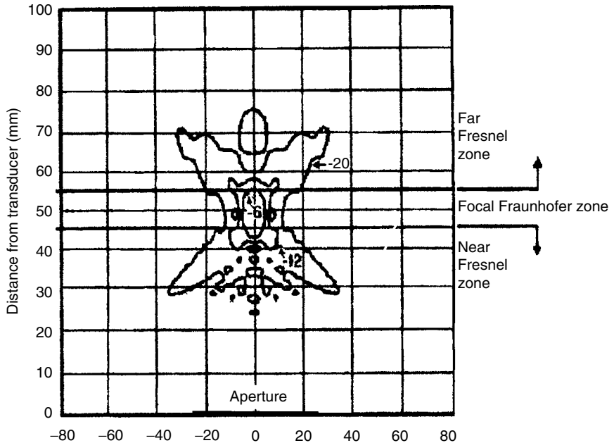
Figure 6.18 Beam contours ( -6 dB, -12 dB, and -20 dB) for a 5-MHz spherically centered aperture at location (0,0) (shown at the bottom center of graph) with a diameter of 25 mm and a radius of curvature of 50 mm. The near Fresnel zone, focal Fraunhofer zone, and far Fresnel zone are marked (from IEC 61828, 2001).
